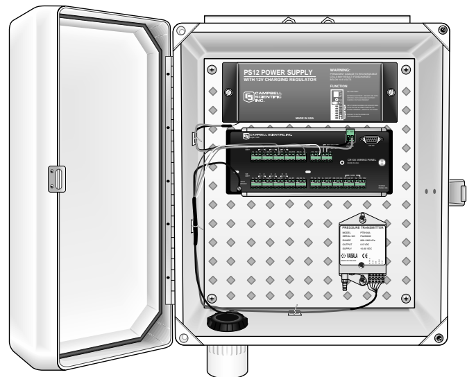
12 Vdc power supply top, CR10X datalogger, and CS105 inside ENC 12/14 enclosure.
