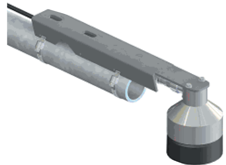
This 19517 mounting assembly is attached directly to a CM206 crossarm via band-clamps.
